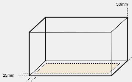
Inside clearance of box less 25mm from outside measurement
