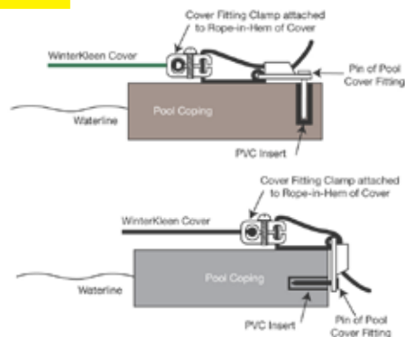
In Ground Option
